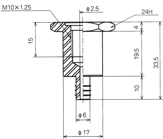
TN-PN-107-M10
