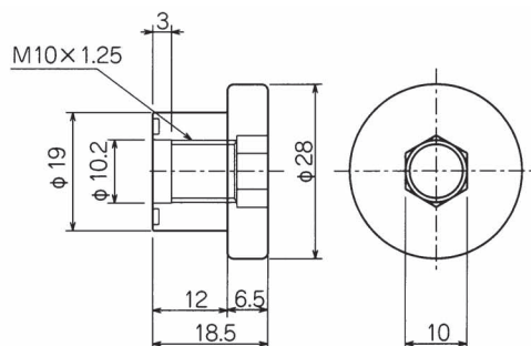
TN-PK-100-M10F
