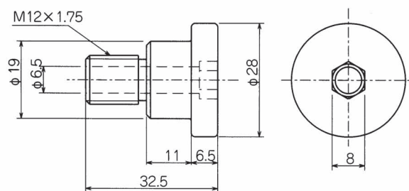
TN-PK-100-M12
