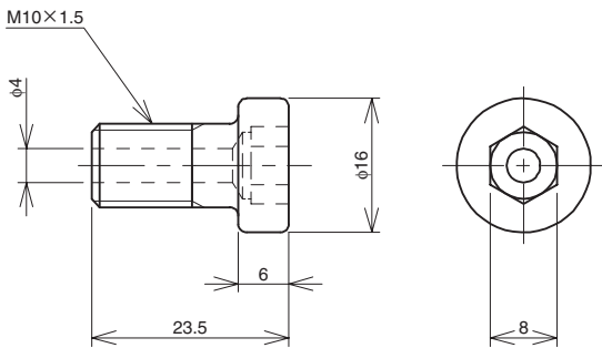
TN-PKM-30-M10
