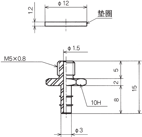
TN-PN-114-M5
